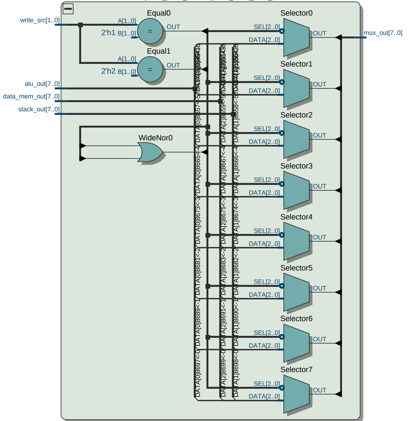
register_write_mux:register_write_mux_inst
