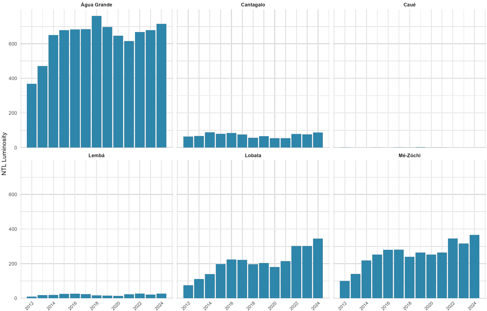
STP - São Tomé : Admin Level 2 Annual Nighttime Lights (2012–2024)
