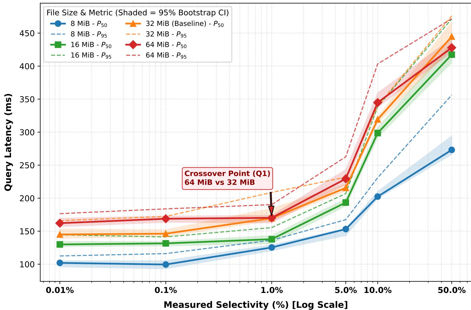
Figure 5: Latency vs. Measured Selectivity — Q1 (Predicate Scan / Lookup)
