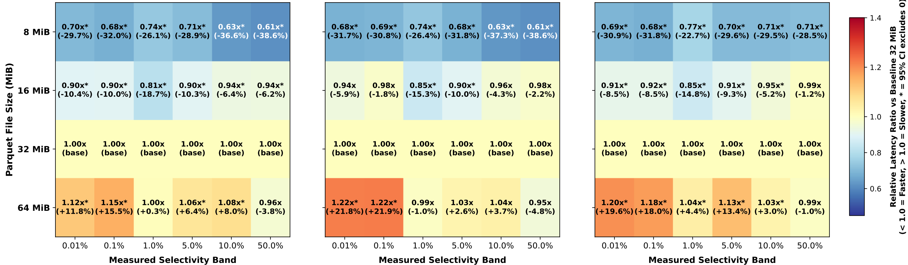
Figure 4: Relative Latency Ratio Heatmap Across Selectivity Bands and File Sizes Q1: Predicate Pushdown (Point / Range Lookup) Q2: Selective Aggregation (AVG / MAX SOG) Q3: Selective Group-By (COUNT by MessageType)
