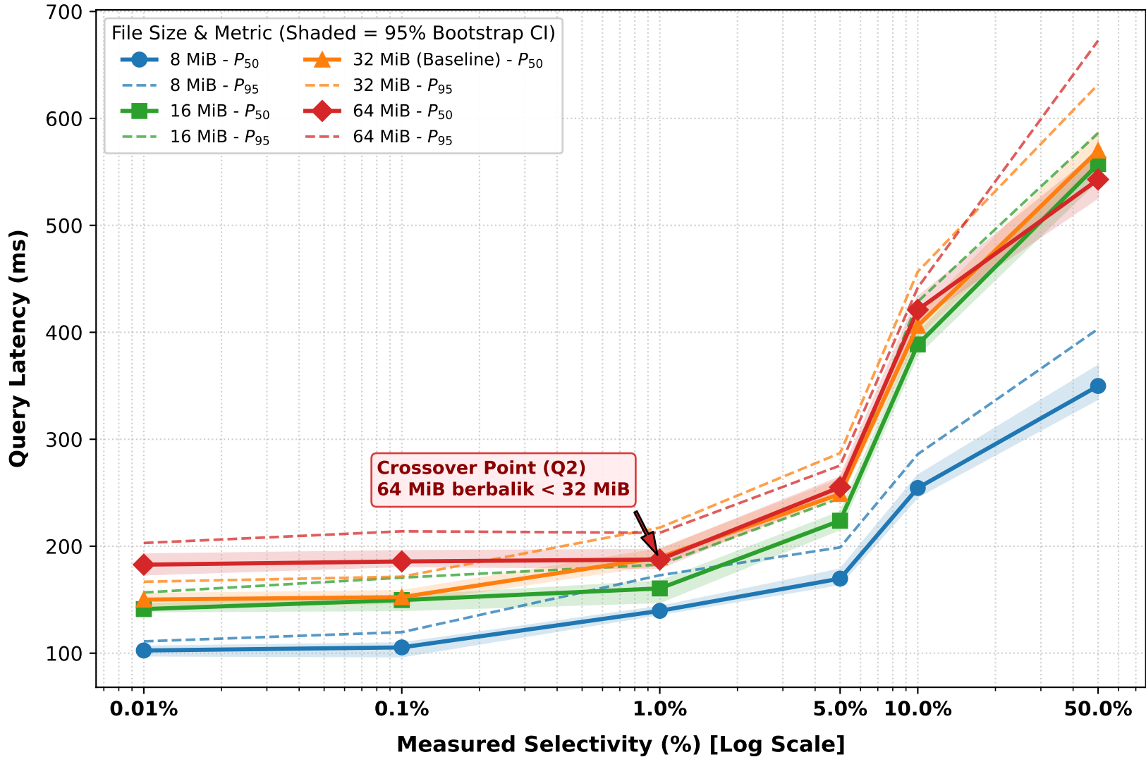
Figure 6: Latency vs. Measured Selectivity — Q2 (Selective Aggregation — SOG AVG/MAX) Evaluates computation overhead atop columnar projection across selectivity bands.
