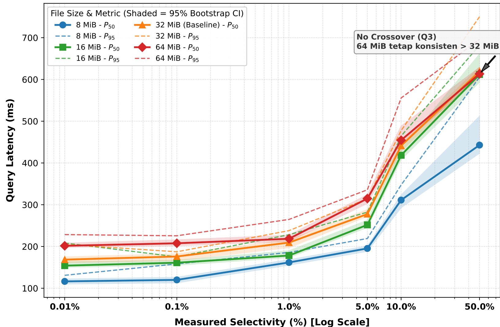
Figure 7: Latency vs. Measured Selectivity — Q3 (Selective Group-By — MessageType) Evaluates partition/hash distribution overhead across file sizes without crossover.
