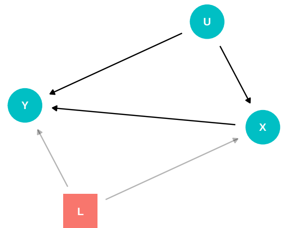
Figure 1: The canonical unobserved confounding DAG. We have measured L , but U , an unmeasured common cause, opening a backdoor path U \rightarrow X \rightarrow Y .
