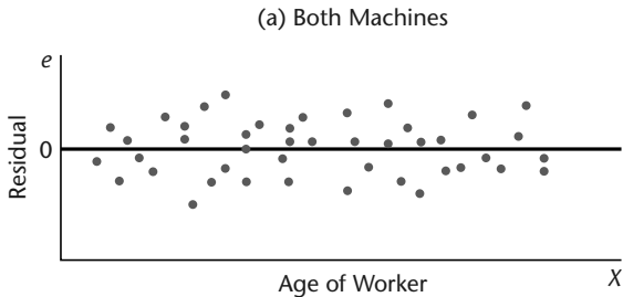
FIGURE 3.10 Residual Plots for Possible Omission of Important Predictor Variable— Productivity Example.
