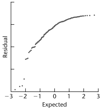
(b) Skewed Left
