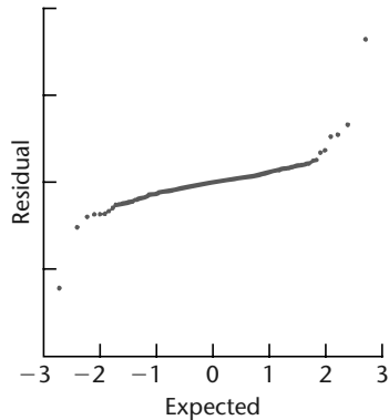
(c) Symmetrical with Heavy Tails
