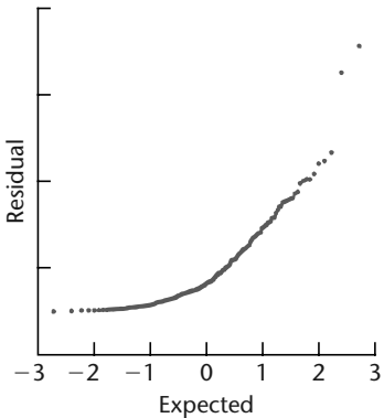
(a) Skewed Right
