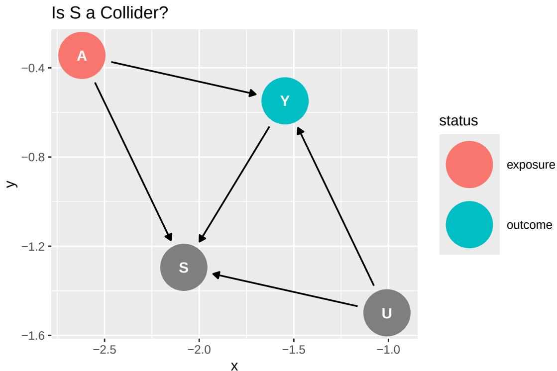
Figure 2: DAG for the Weight Loss App Selection Bias Scenario
