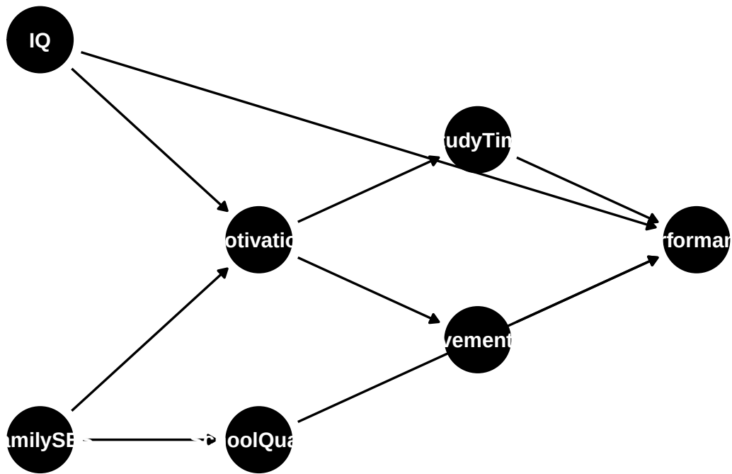
Student Performance Causal DAG
