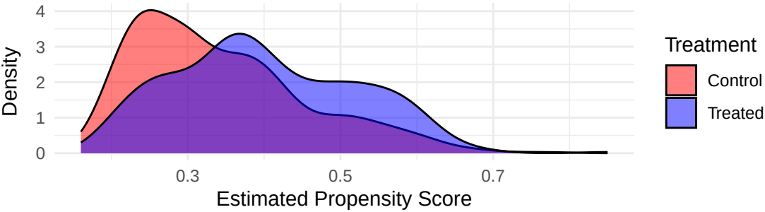
Propensity Score Densities
