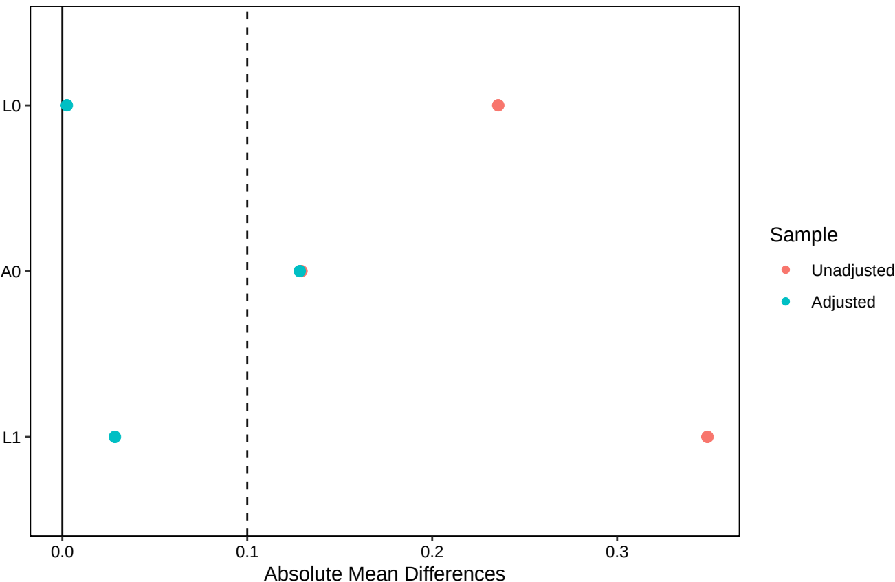
Covariate Balance Max across time points
