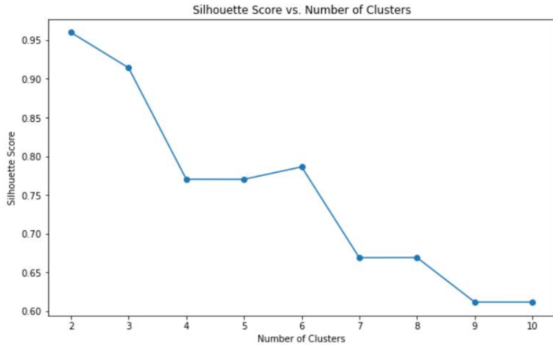
Silhouette Score vs. No. of Clusters
