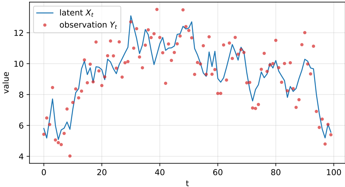
Latent state X_t and noisy observation Y_t = X_t + e_{2,t}
