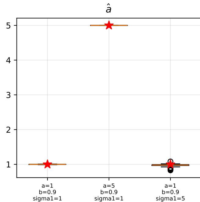
MLE estimates across 3 parameter configurations (100 reps each, red star = truth)
