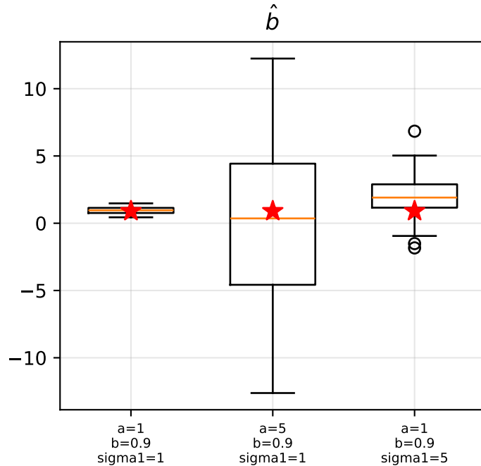
MLE estimates across 3 parameter configurations (100 reps each, red star = truth)
