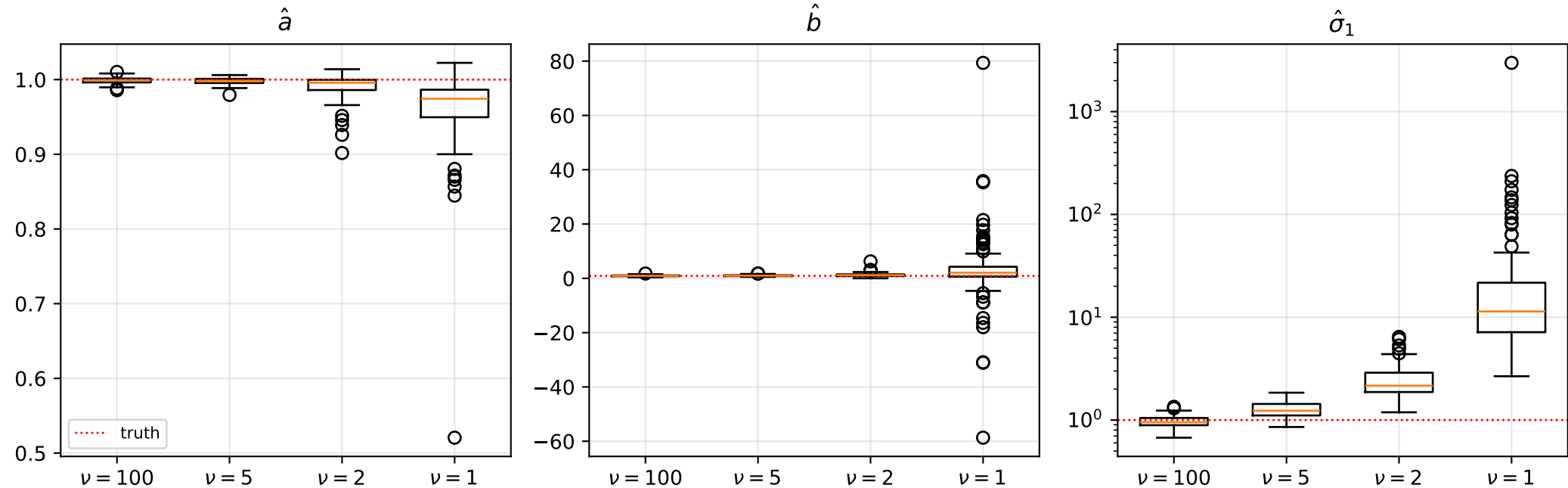
Gaussian-KF MLE estimates under Student- t process noise
