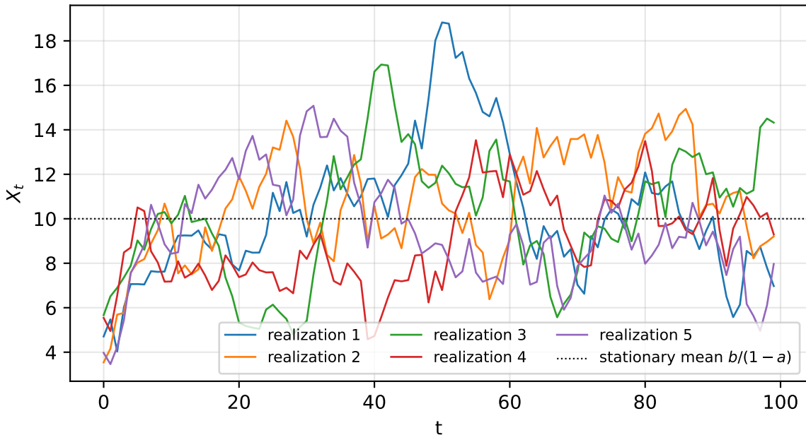
Five independent realizations of the latent process
