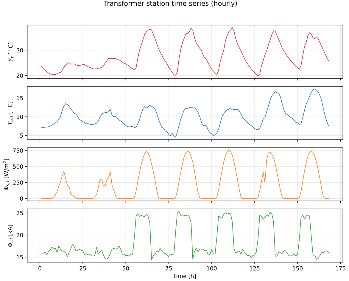
Figure 7: Transformer temperature Y_t , outdoor temperature T_{a,t} , solar radiation \Phi_{s,t} and load \Phi_{I,t} (hourly, one week).
