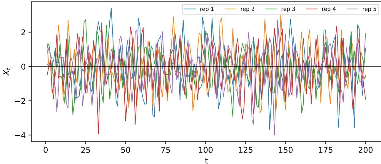
AR(2) simulations — \phi_1 = -0.6 , \phi_2 = 0.5
