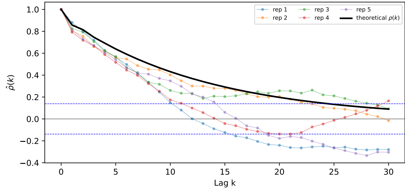
Empirical ACF — \phi_1 = -0.6, \phi_2 = -0.3
