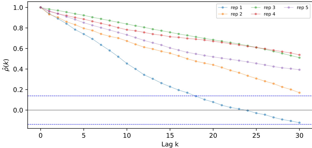
Empirical ACF — \phi_1 = -0.7, \phi_2 = -0.3 [NON-STATIONARY, no theoretical ACF]
