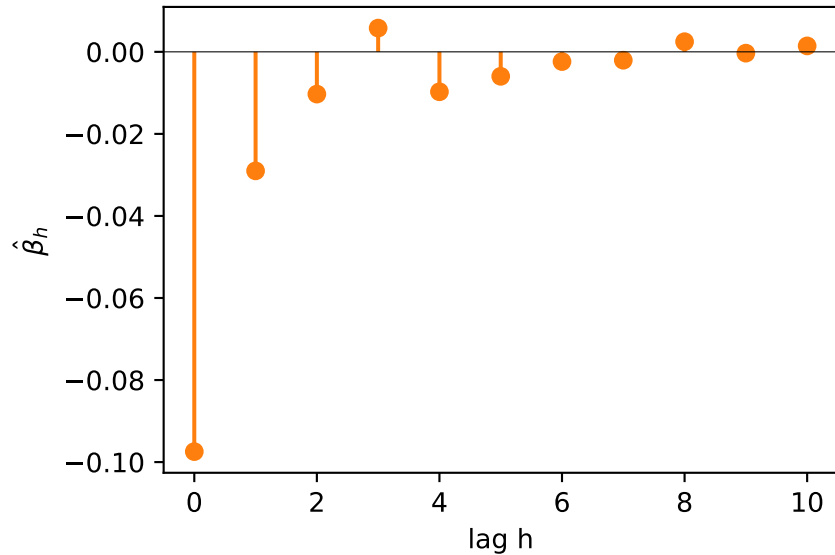
Impulse response G_V \rightarrow \text{Ph}
