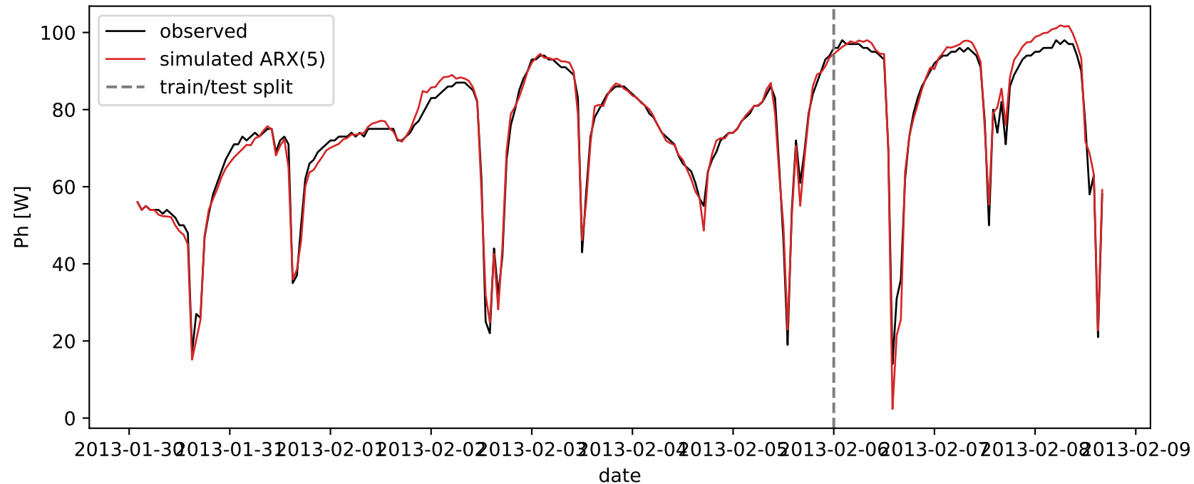
3.9 Multi-step simulation (ARX(5), inputs observed)
