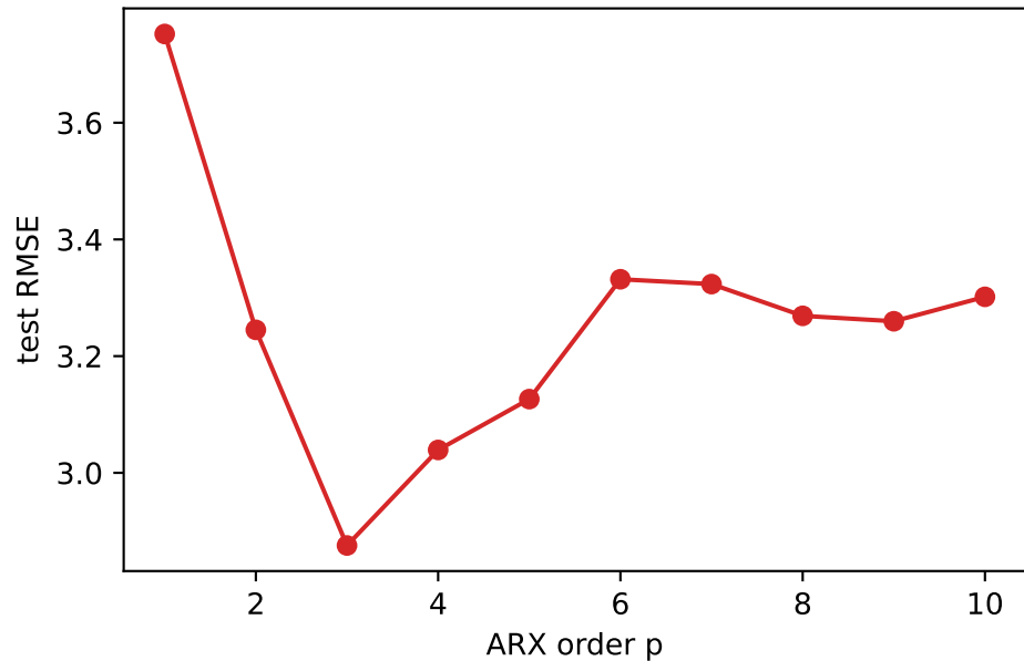
One-step test RMSE vs ARX order
