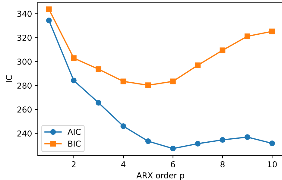
AIC / BIC vs ARX order
