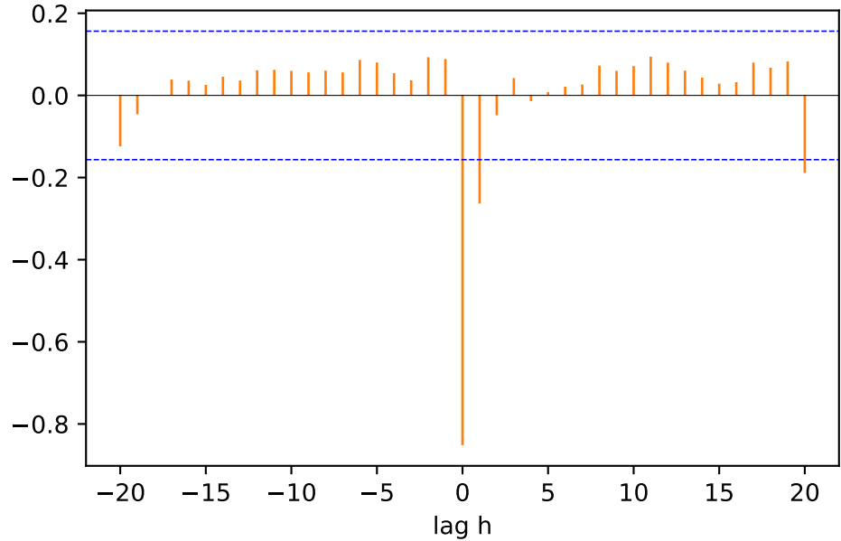
Pre-whitened CCF ( G_v \rightarrow \text{Ph} ), AR(10)
