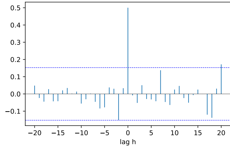
Pre-whitened CCF ( T_\Delta \rightarrow \text{Ph} ), AR(2)
