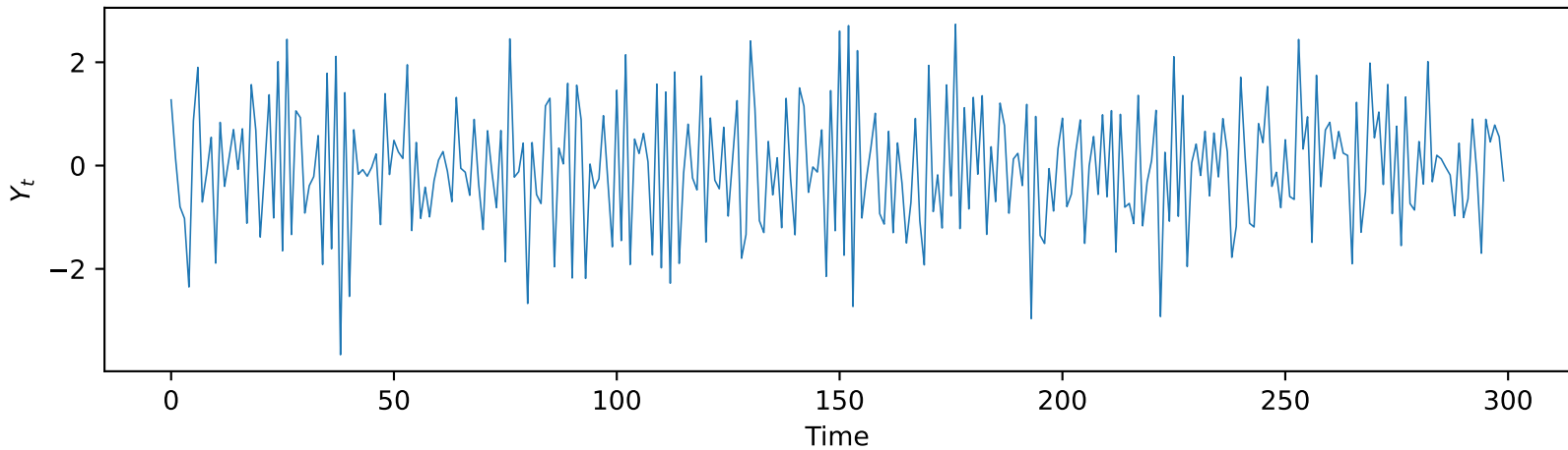
Model 2.1: (1, 0, 0) \times (0, 0, 0)_{12} , \phi_1 = 0.6
