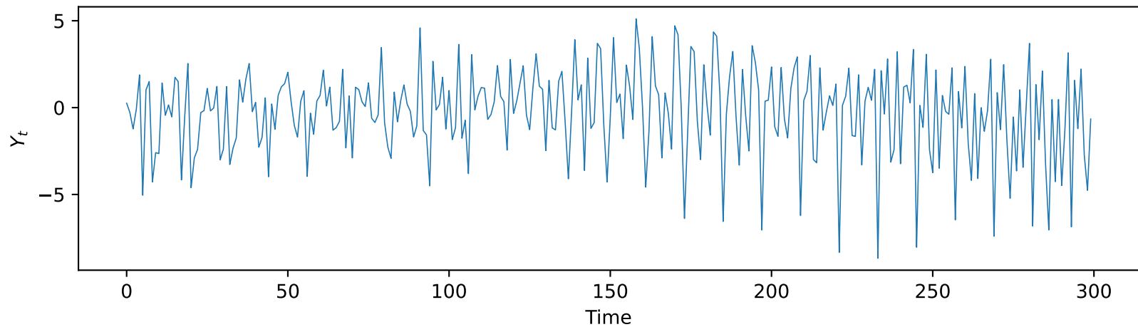
Model 2.2: (0, 0, 0) \times (1, 0, 0)_{12} , \Phi_1 = -0.9
