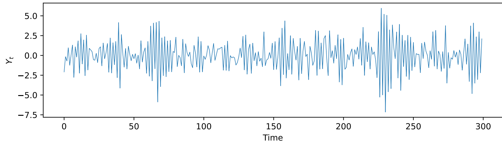
Model 2.3: (1, 0, 0) \times (0, 0, 1)_{12} , \phi_1 = 0.9 , \Theta_1 = -0.7
