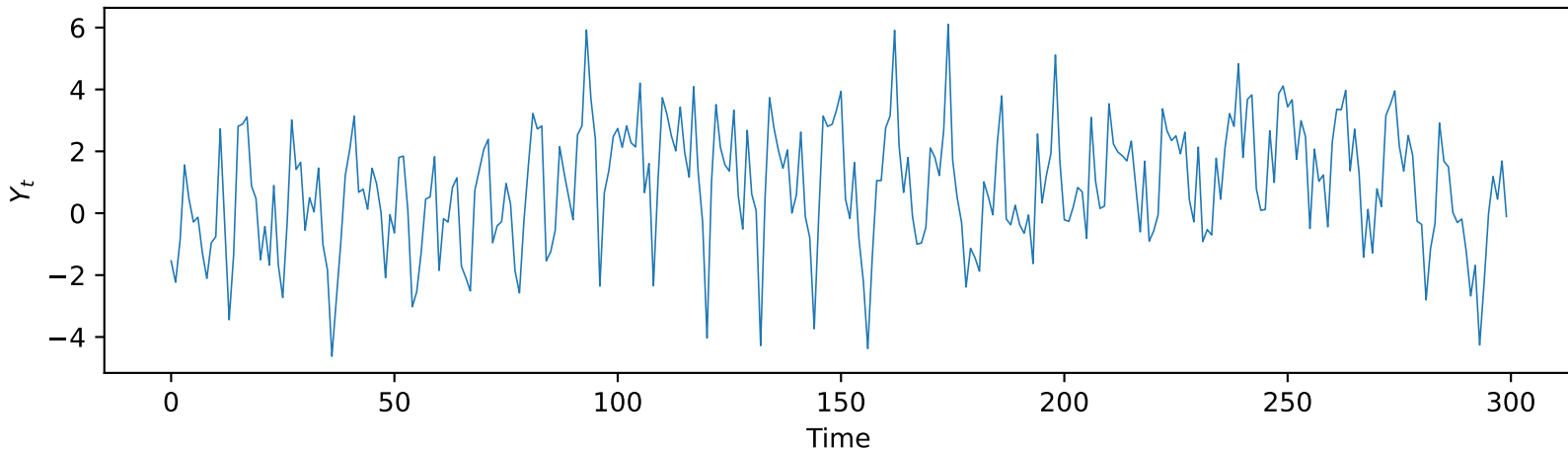
Model 2.4: (1, 0, 0) \times (1, 0, 0)_{12} , \phi_1 = -0.6 , \Phi_1 = -0.8
