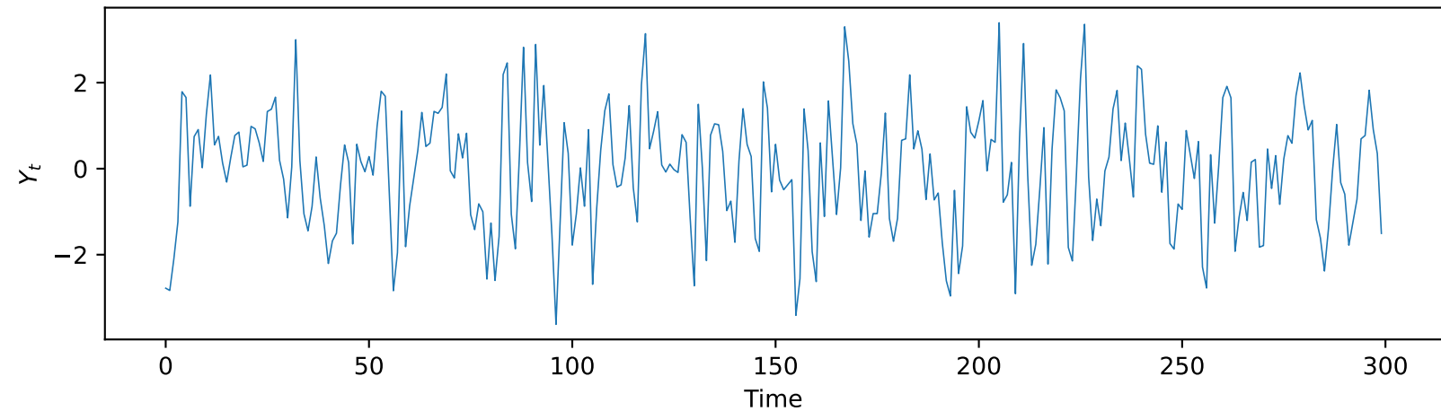
Model 2.5: (0, 0, 1) \times (0, 0, 1)_{12} , \theta_1 = 0.4 , \Theta_1 = -0.8
