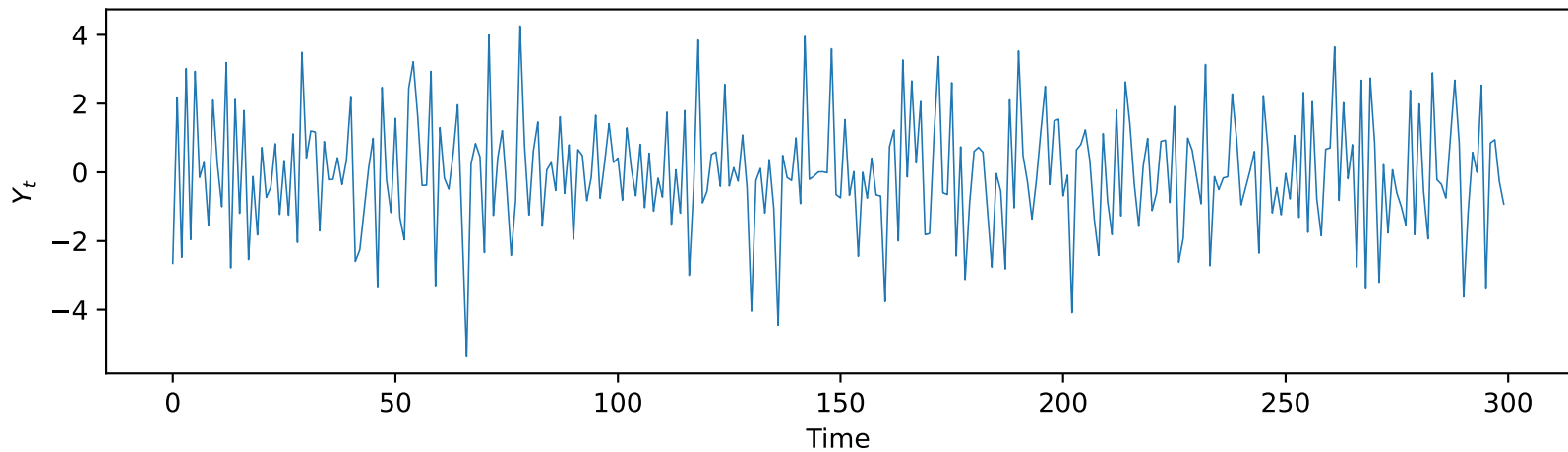
Model 2.6: (0, 0, 1) \times (1, 0, 0)_{12} , \theta_1 = -0.4 , \Phi_1 = 0.7
