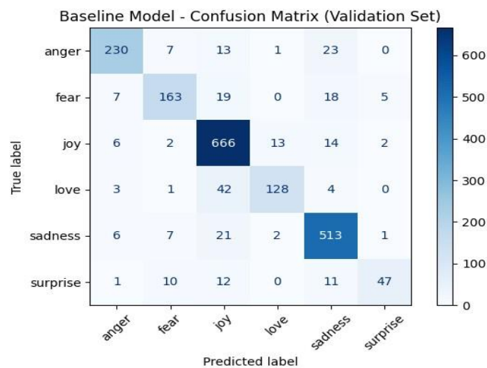
Fig. 2.2.1 Confusion Matrix (Baseline Model)
