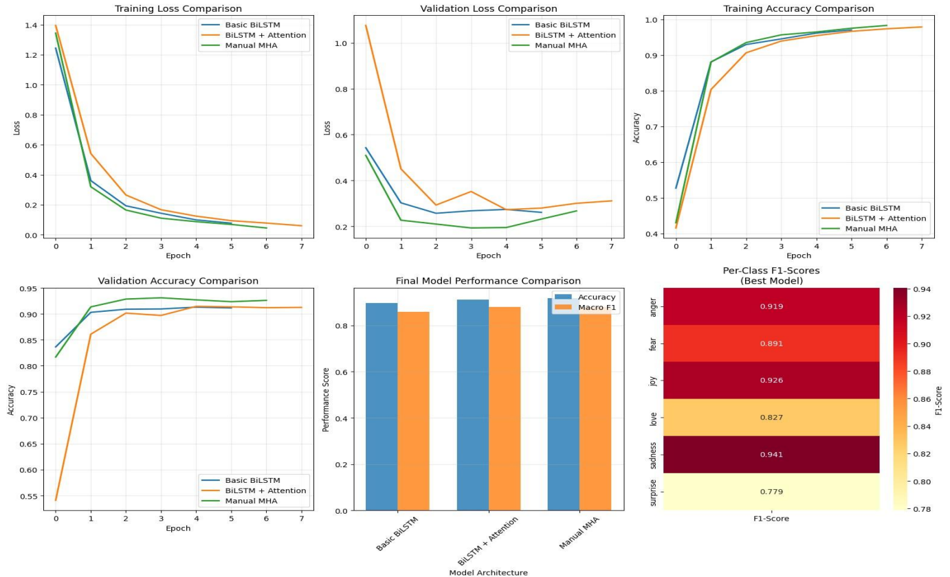
Fig. 2.3.1 DL Model Comparison
