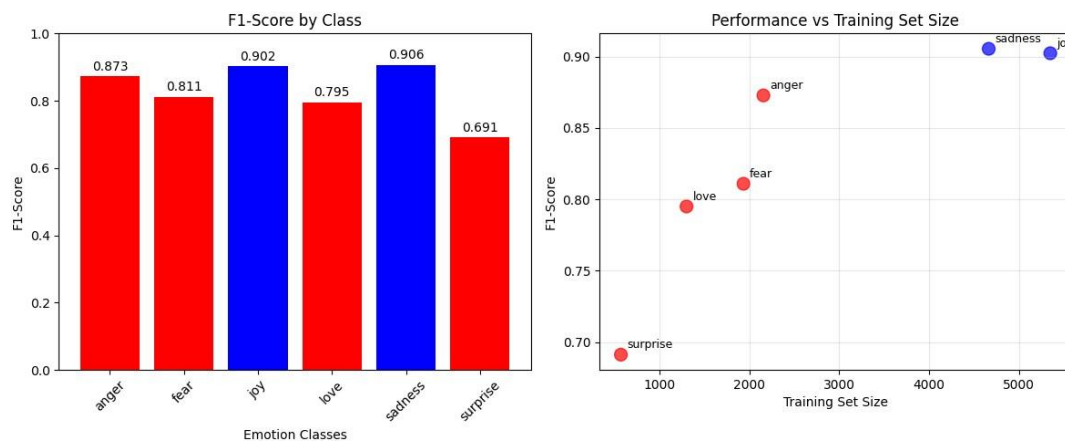
Fig. 2.2.2 Baseline Model Performance
