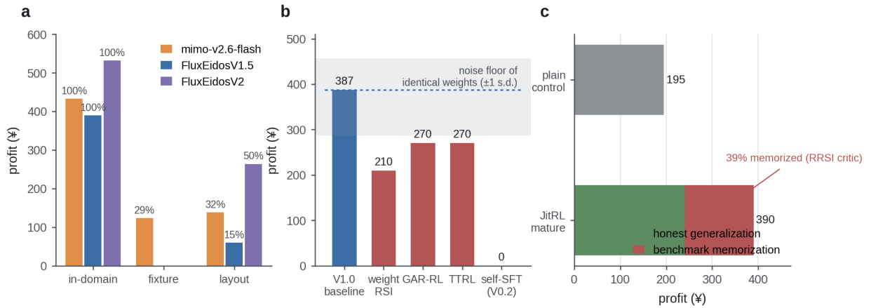
Figure 3: Figure 3 | The three failures. (a) Domain shift degrades everyone — the frontier retains 29–32% of in-domain profit (3-judge, n=5/\text{cell} ). (b) All four weight-level self-improvement families fall below the trained baseline and inside the noise floor of identical weights (gray band: \pm 1 sd of repeated evaluation). (c) Cross-session experience gain decomposes into honest generalization (¥240) and benchmark memorization (¥150, 39%) under RRSI-style regularization.
