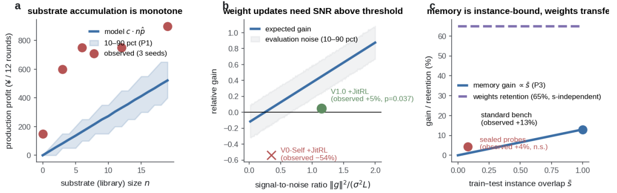
Figure 5: Figure 5 | Minimal formal model vs. empirics. Left (P1): substrate accumulation is monotone — model expectation with 10-90 pct band overlaid with the observed library dose-response (3 seeds). Middle (P2): weight updates need SNR above a threshold; shaded band is evaluation noise, with observed below-threshold (V0-Self, -54%) and above-threshold (V1.0, +5%) anchors. Right (P3): memory gain scales with train-test overlap \bar{s} whereas weights transfer with s-independent retention — observed on-distribution (+13%) and sealed-probe (+4%, n.s.) points.
