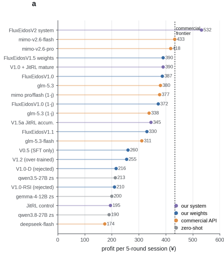
Figure 2: Figure 2 | Main ranking (profit per 5-round session). Our system entries (purple) and weights (blue) against commercial APIs (orange) and zero-shot open models (gray); 14 zero-shot systems at ¥0 omitted for space. Dotted line marks the commercial frontier.
