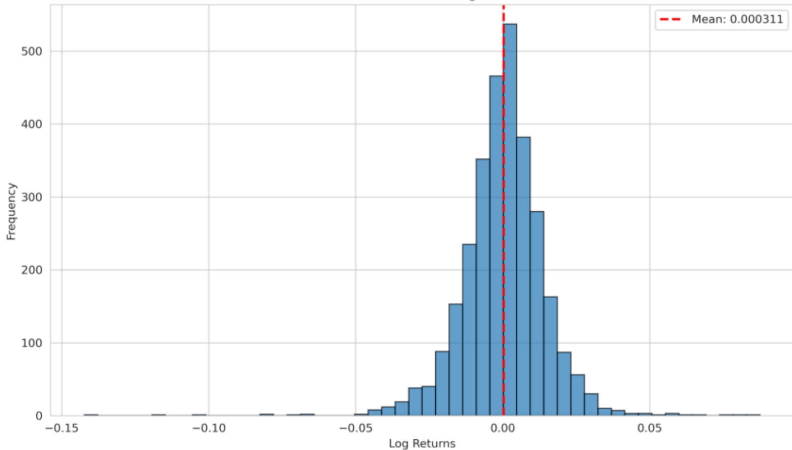
Distribution of 1-Bar Log Returns
