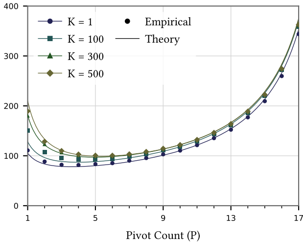
Expected Listwise Ranker Calls
