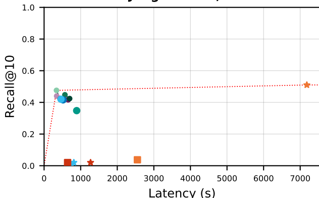
LLM-as-Judge Labels, Selection
