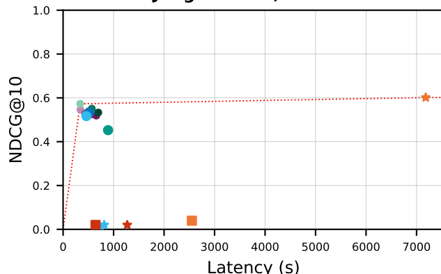
LLM-as-Judge Labels, Selection+Sort
