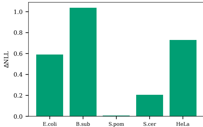
Unified advantage
