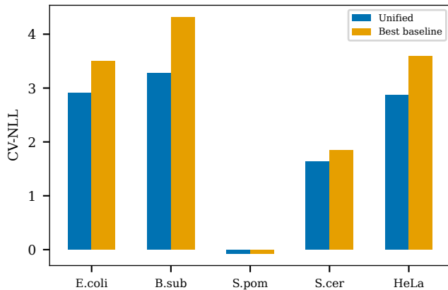
Cross-validated NLL
