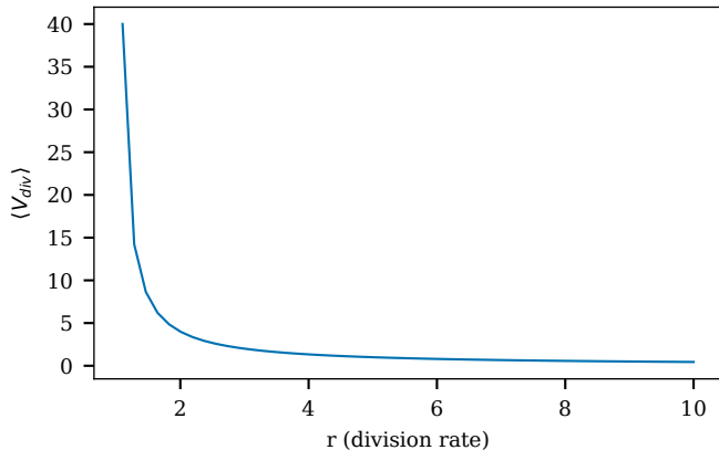
CDK4/6i effect
