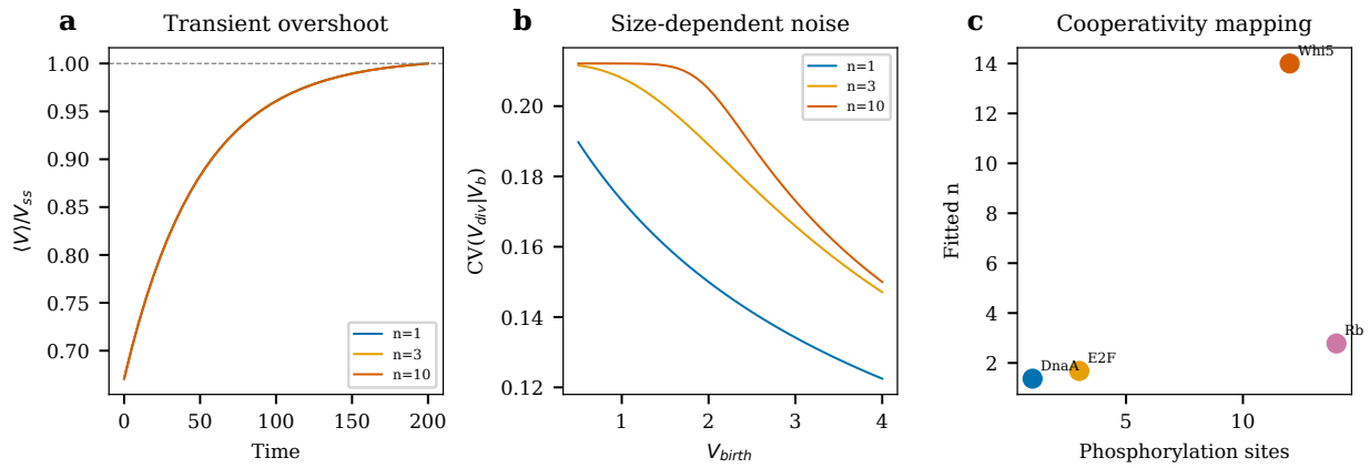
Figure 4: Figure 4 | Novel predictions beyond existing models. a , Predicted transient overshoot in mean cell size after nutrient upshift, for different n values. b , Birth-size-dependent conditional CV of division size: CV(V_{\text{division}} | V_{\text{birth}}) \propto (V_{\text{birth}}^n + K^n)^{-1/(2n)} . c , Mapping Hill coefficient n to molecular cooperativity: predicted versus measured phosphorylation sites for Whi5 and Rb.
