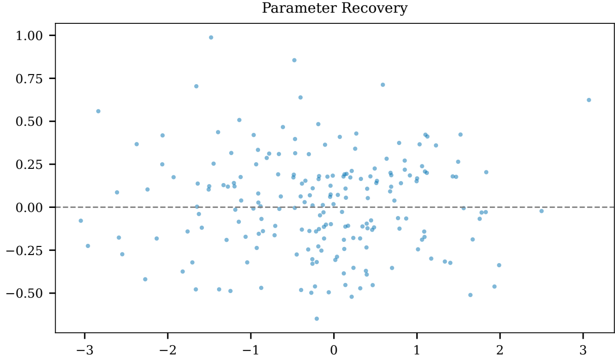
Figure 8: Extended Data Fig. 3 | Parameter recovery from simulated data. Parameters (n, K, r) estimated from synthetic data generated with known ground truth, demonstrating accurate and unbiased recovery across all parameter regimes.
