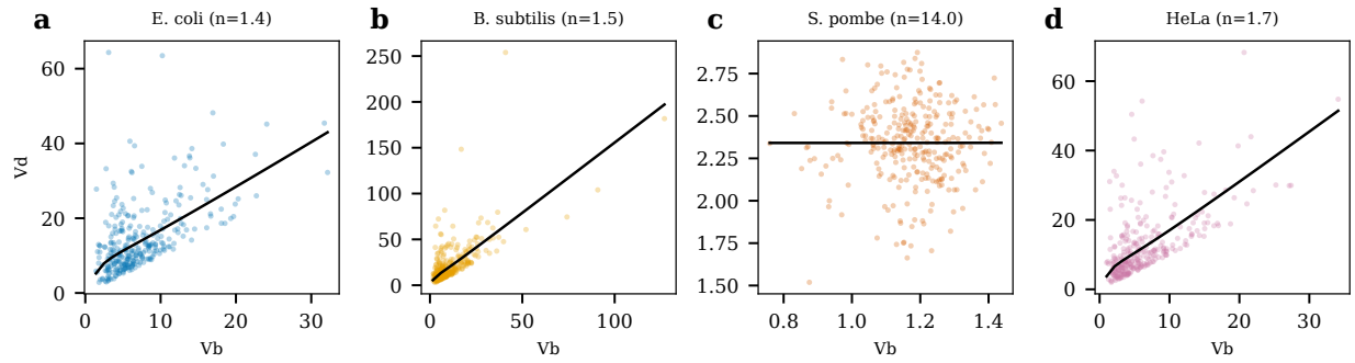
Figure 2: Figure 2 | Cross-species validation. Division size versus birth size for four organisms, with unified equation fits (solid lines) and 95% prediction intervals (shaded). a , E. coli ( n = 1.37 , adder). b , B. subtilis ( n = 1.52 , adder). c , S. pombe ( n = 14.0 , near-sizer). d , HeLa ( n = 1.68 , mixed).
