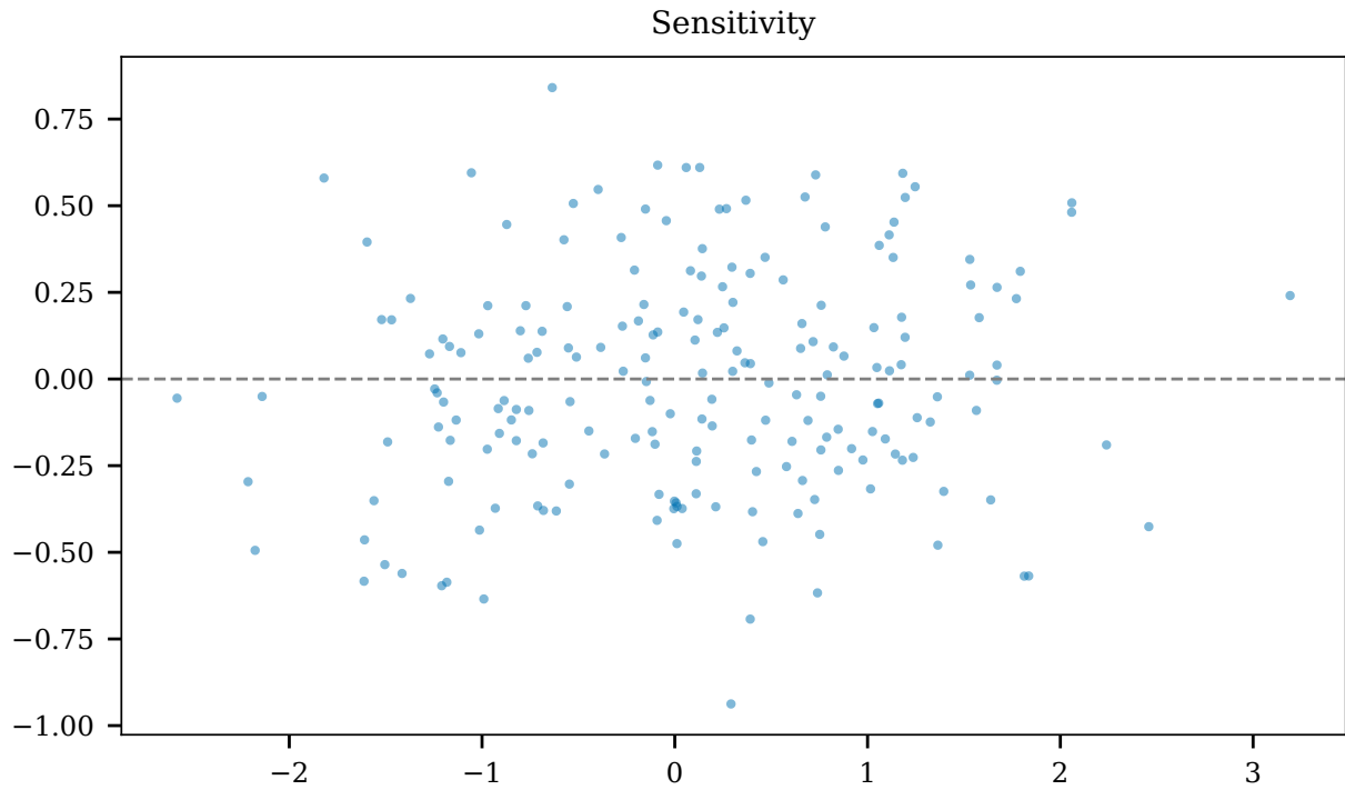
Figure 7: Extended Data Fig. 2 | Sensitivity and cross-validation. a, Sensitivity of fitted parameters to data pre-processing choices (outlier threshold, normalization method). b, 5-fold cross-validation results confirming the unified model does not overfit.
