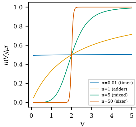
Hill function
