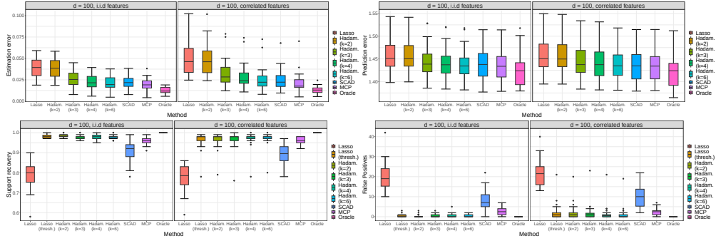
Fig. B3: Left: standardized estimation error (top row) and (test) support recovery (bottom row) for different \Sigma settings (columns) of our approach for increasing factorization depths, compared against standard implementations of convex \ell_1 and non-convex SCAD and MCP penalties. Right: prediction error (top row) and false positives (bottom row) for different settings of \Sigma (columns).
