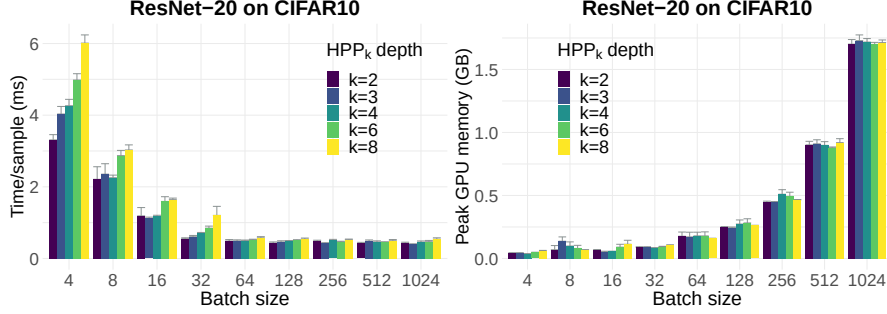
Fig. B4: Left: training time per sample for different factorization depths k . Right: peak GPU memory utilization. Means and standard errors over four runs are displayed.
