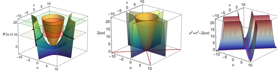
(a) Optim. Transfer (HPP)
