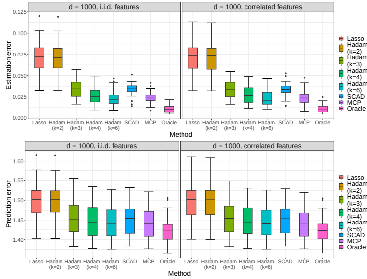
Fig. 7: Stand. estimation error (top row) and test prediction error (bottom row) for two \Sigma settings (columns) of our approach for depths k \in \{2, 3, 4, 6\} , compared with specialized optimizers for \ell_1 and non-convex SCAD and MCP penalties.
