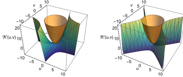
Fig. C5: Left: HPP (blue/green) and the surrogate \ell_2 regularization u_j^2 + v_j^2 (orange). Right: HDP (blue/green) and surrogate \ell_2 regularization.
