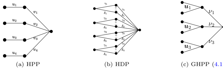
Fig. 3: Diagonal linear networks corresponding to different parametrizations of a linear predictor: a) HPP ( \ell_1 ), b) HDP ( \ell_1 ), c) Structure-inducing parametrization (GHPP for \ell_{2,1} , cf. 4.1) with grouping layer. Left nodes are inputs, and the right-most node the output.
