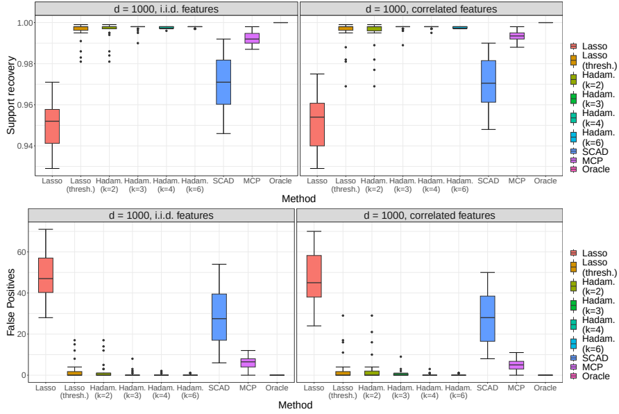
Fig. B2: Support recovery accuracy (top row) and false positives (bottom row) for different \Sigma settings (columns) and increasing factorization depths, compared against standard implementations of convex \ell_1 and non-convex SCAD and MCP penalties.
