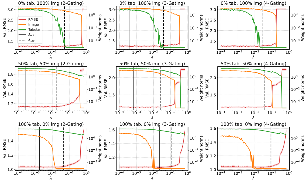
Figure 20: Regularization path and weight norms in multi-modal late-fusion network for different modality contributions ( rows ) and D -Gating depth D \in \{2, 3, 4\} ( columns ). The solid vertical bar indicates the validation-optimal \lambda_{opt} and the dashed vertical bar the \lambda_{1se} chosen by the 1se rule, i.e., the sparsest model that performs within one standard error of the lowest validation RMSE (10 splits).
