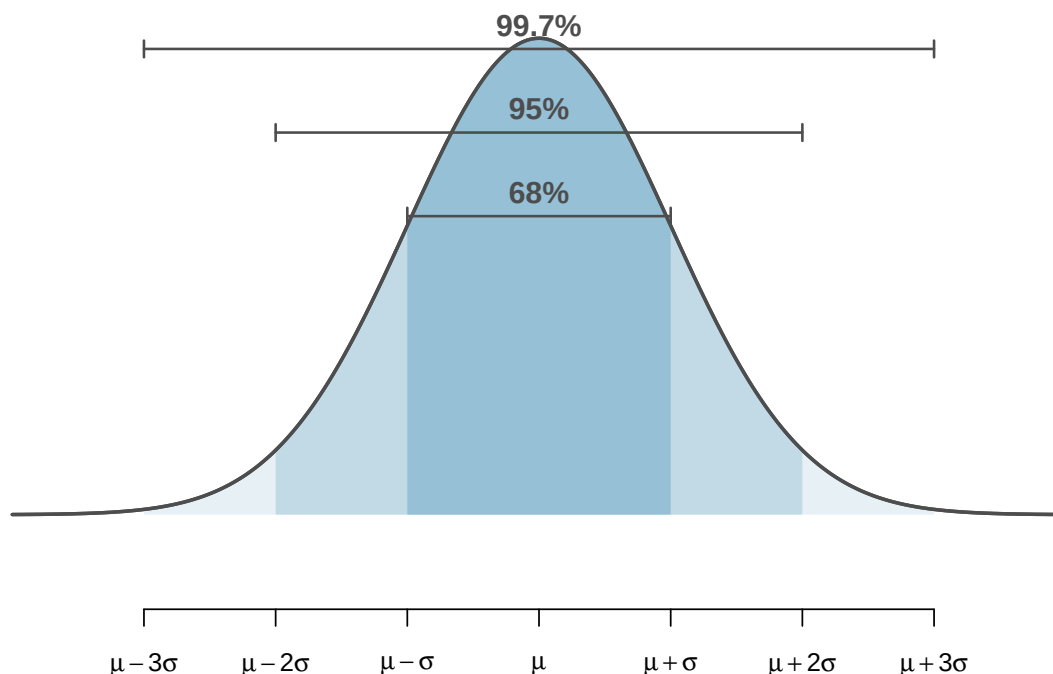
Figure 10.1: The 68-95-99.7 rule for normal distributions. Approximately 68% of values fall within 1 standard deviation of the mean, 95% within 2, and 99.7% within 3. ↗ Try this live — drag the cutlines to see the 68-95-99.7 boundaries live.
