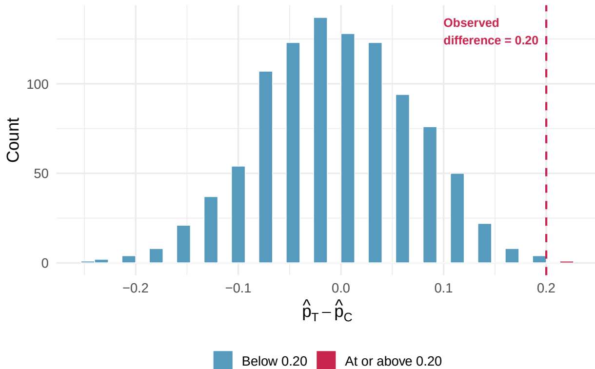
Figure 1: A histogram of 1,000 simulated differences produced under the null hypothesis. Differences at least as large as the observed 0.20 are highlighted in red.
