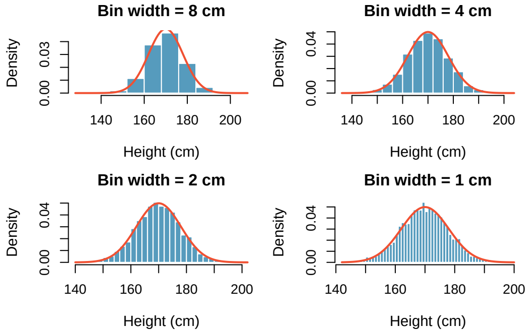
Figure 24.2: The transition from a histogram to a smooth density curve as the bin width decreases and sample size increases.
