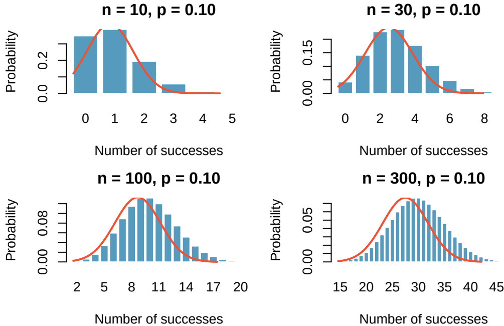
Figure 26.1: Binomial distributions with p = 0.10 and sample sizes n = 10, 30, 100 , and 300 . As n increases, the distribution approaches a normal curve.
