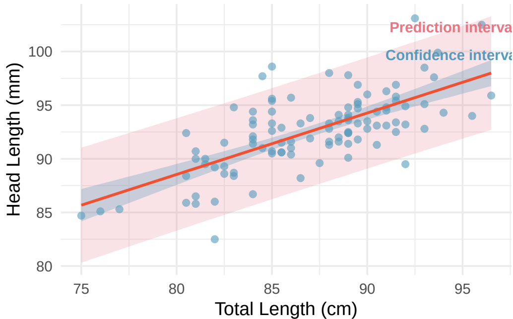
Figure 22.4: A scatterplot with a regression line and both 95% confidence bands (narrow) and 95% prediction bands (wide). Both bands are narrowest near the mean of x and flare outward.
