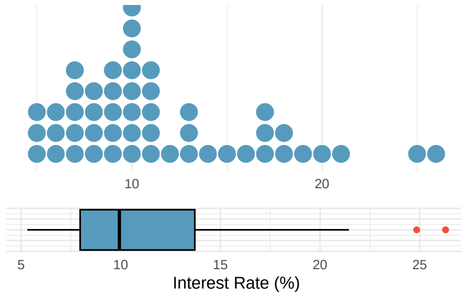
Figure 14: A dot plot and box plot of the same interest rate data, shown one above the other for comparison. The box plot summarizes the distribution with five numbers plus outliers.
