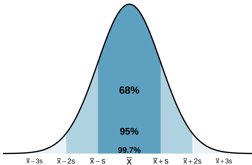
Figure 16: A bell-shaped distribution with shaded regions showing 68%, 95%, and 99.7% of the data within 1, 2, and 3 standard deviations of the mean, respectively.
