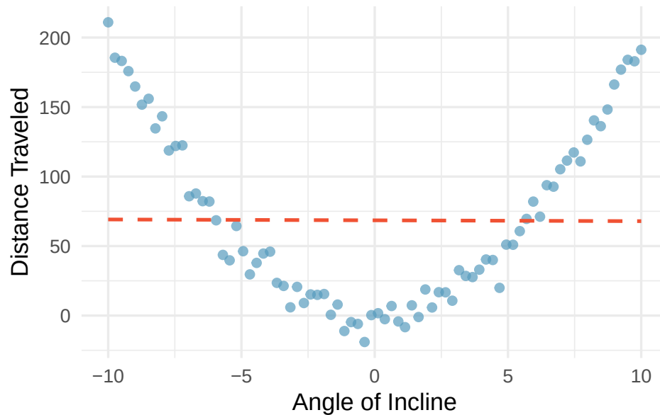
Figure 36: A scatterplot showing a clear quadratic (U-shaped) relationship between angle of incline and distance traveled. The best-fitting straight line is flat and does not capture the pattern at all.
