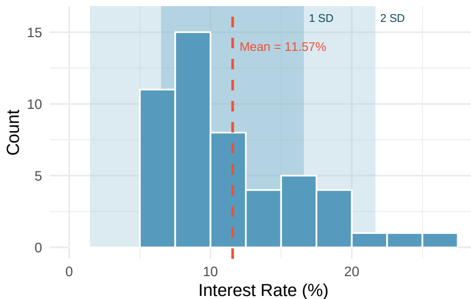
Figure 13: A histogram of interest rates with shaded regions showing one standard deviation (dark) and two standard deviations (light) from the mean.
