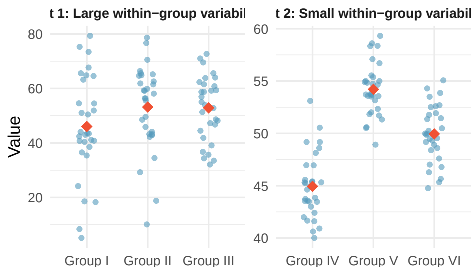
Figure 34: Side-by-side dot plots for two sets of three groups. In the first set (Groups I, II, III), the within-group variability is large relative to the between-group differences. In the second set (Groups IV, V, VI), the within-group variability is small and the between-group differences are clearly visible.
