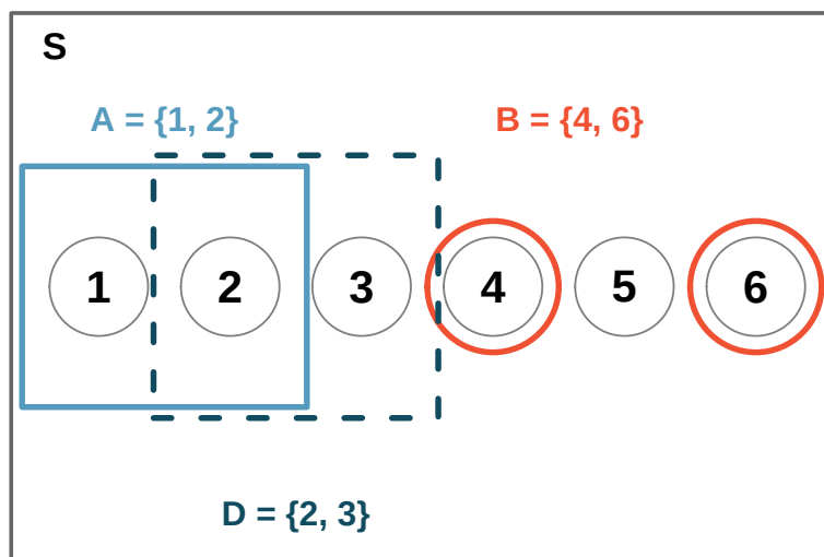
Figure 42: Three events for die outcomes. A and B are disjoint since they share no outcomes.
