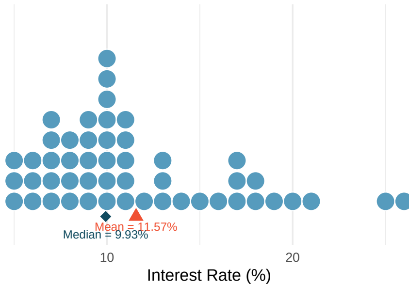
Figure 12: A dot plot of interest rates with the mean (red triangle, 11.57%) and median (blue diamond, 9.93%) marked. The mean is pulled to the right by the high-interest loans.
