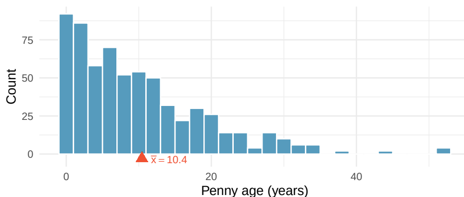
Figure 26: Distribution of ages for 648 pennies sampled from circulation. The distribution is right-skewed with a mean of about 10.4 years. The sample mean is marked with a red triangle. Open in StatLens
