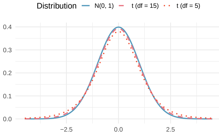
Figure 32: Three distributions plotted on the same axes: the standard normal distribution N(0, 1) , a t -distribution with df = 5 , and a t -distribution with df = 15 . All are centered at 0 and bell-shaped, but the t -distributions have heavier tails, especially when df is small.
