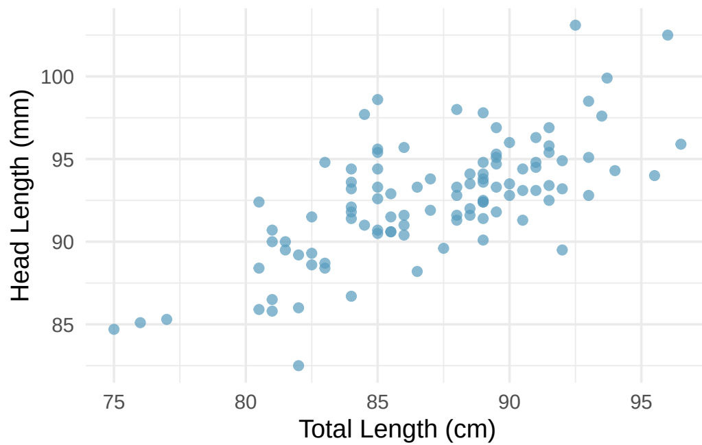
Figure 35: A scatterplot showing head length against total length for 104 brushtail possums. The relationship is moderately strong, positive, and linear.
