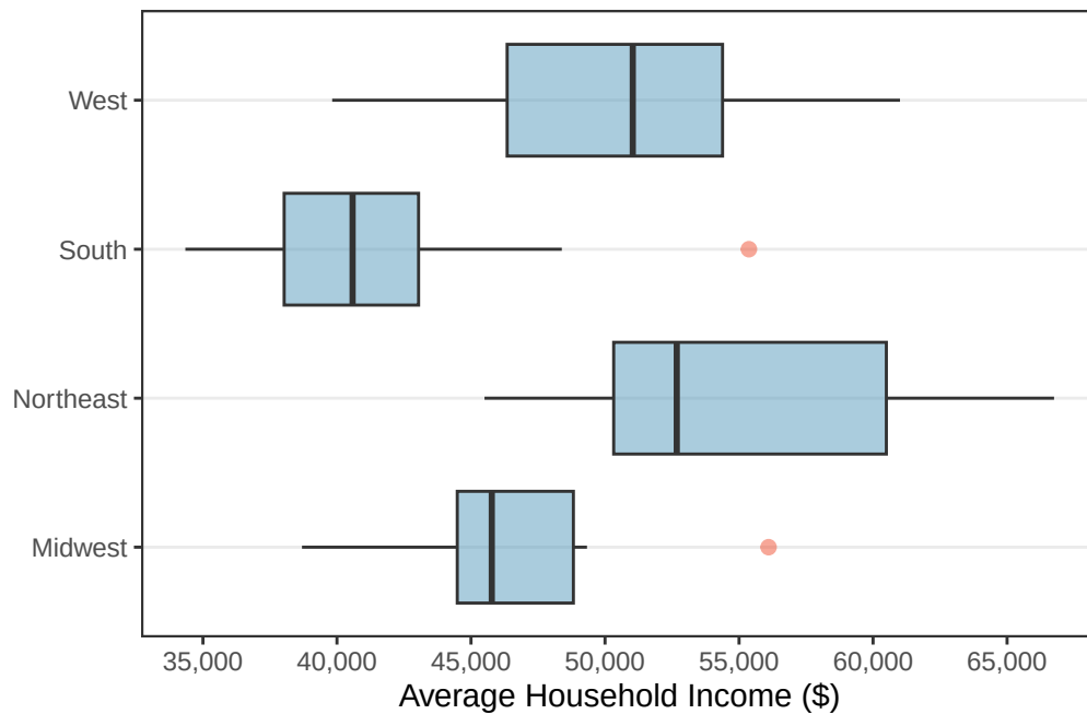
Figure 17: A side-by-side box plot of average household income split by geographic region in the US.
