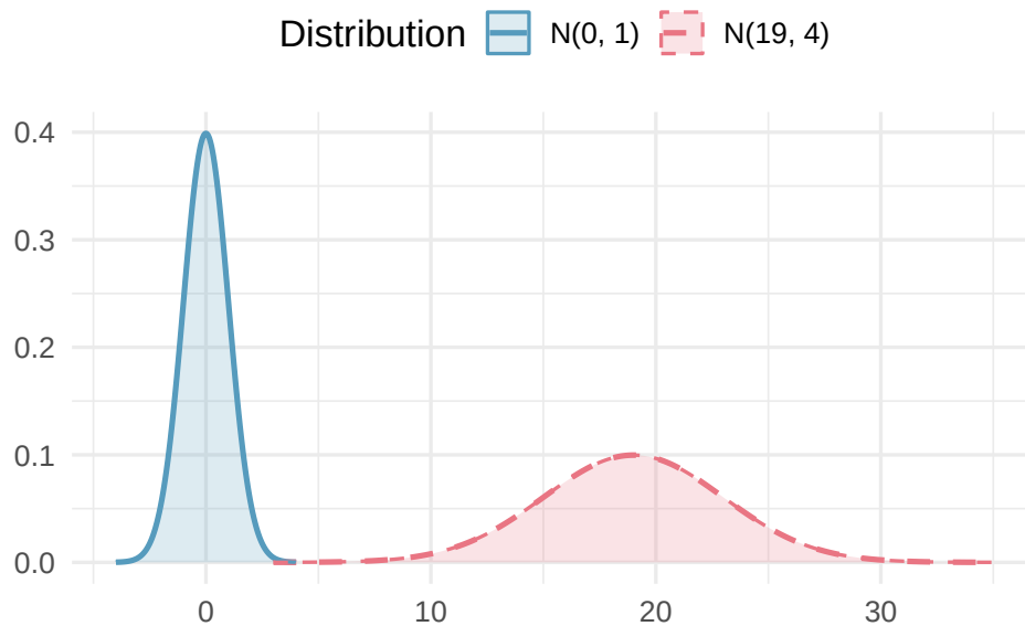
Figure 30: Two normal distributions with different parameters. The left curve has \mu = 0 and \sigma = 1 ; the right curve has \mu = 19 and \sigma = 4 . Changing \mu shifts the curve left or right; changing \sigma stretches or compresses it.
