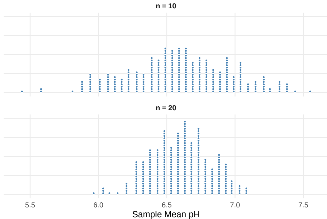
Figure 20: Two sampling distributions for average pH levels in Florida lakes.
