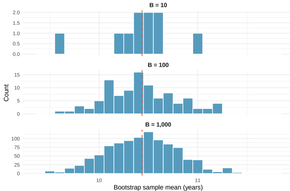
Figure 27: Building up the bootstrap distribution. With 10 resamples we see only a rough sketch; by 1,000 resamples the shape of the distribution is clear — and approximately bell-shaped (normal), even though the original data are skewed.
