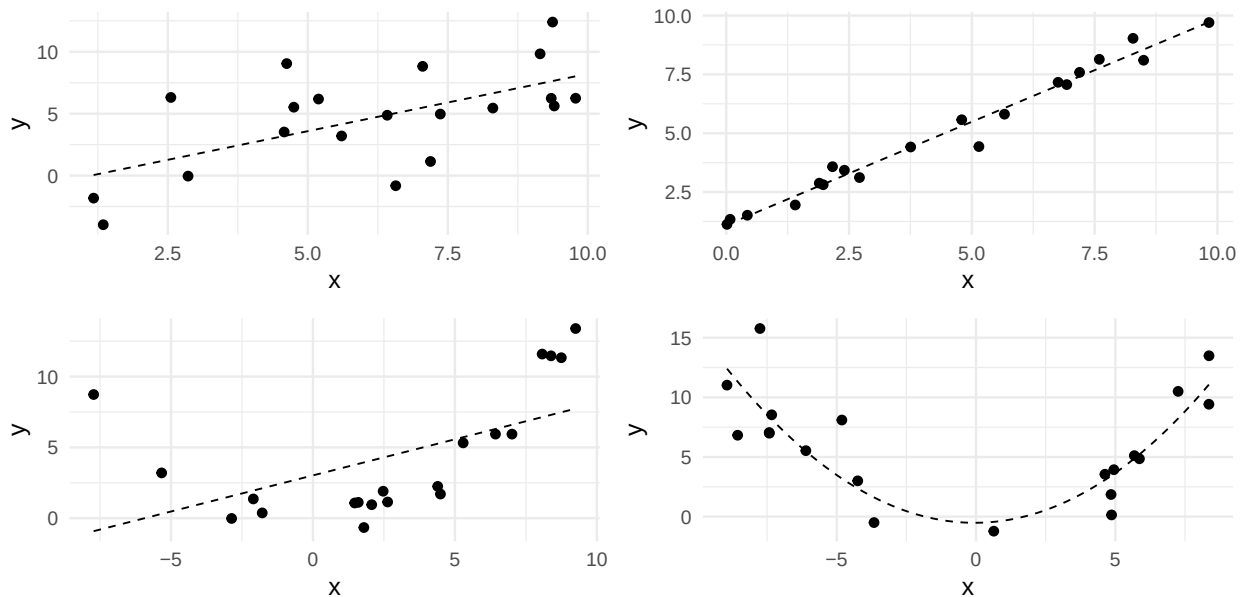
Figure 39: Four scatterplots with fitted regression model fit to the data.
