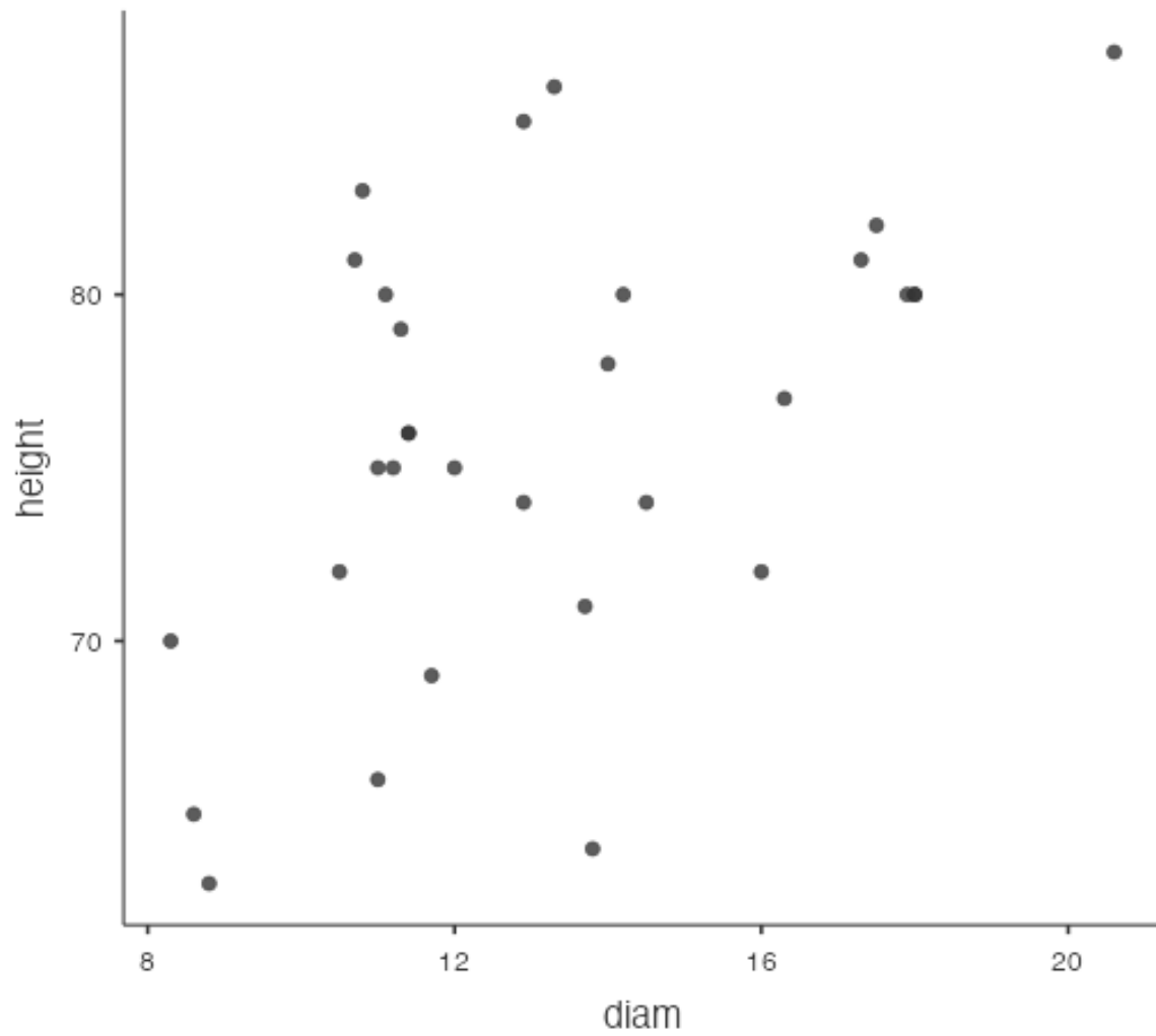
Figure 41: Scatterplot of the height and diameter of the cherry trees.
