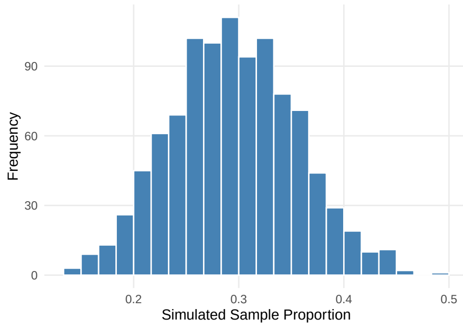
Figure 22: Randomization distribution with 1000 randomizations
