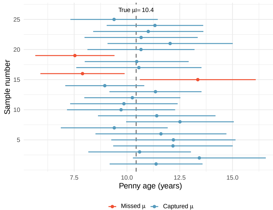
Figure 24: Twenty-five 95% confidence intervals from 25 different random samples of pennies. The true population mean is shown as a vertical dashed line. Approximately 95% of intervals capture the true mean; a few (shown in red) miss it.
