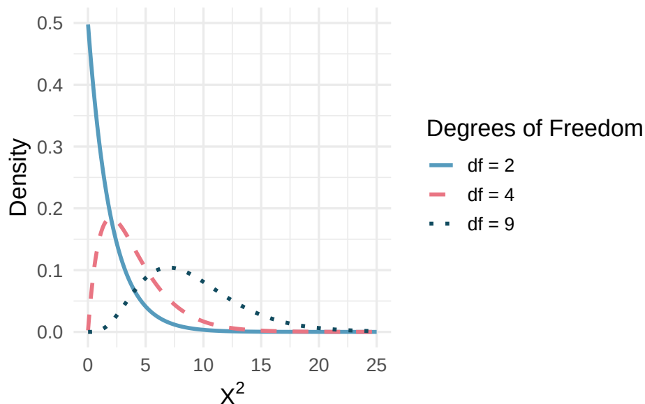
Figure 33: Three chi-square distributions with degrees of freedom 2, 4, and 9. As the degrees of freedom increase, the distribution becomes more symmetric, the center moves to the right, and the variability increases.
