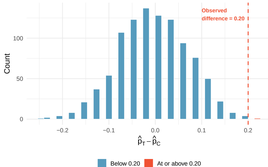
Figure 21: A histogram of 1,000 simulated differences produced under the null hypothesis. Differences at least as large as the observed 0.20 are highlighted in red.
