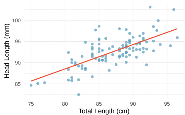
Figure 38: A scatterplot showing head length against total length for 104 brushtail possums, with a linear model fit to the data.
