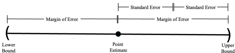
Figure 25: Diagram of the relationship between the 95% confidence interval, margin of error, and standard error.
