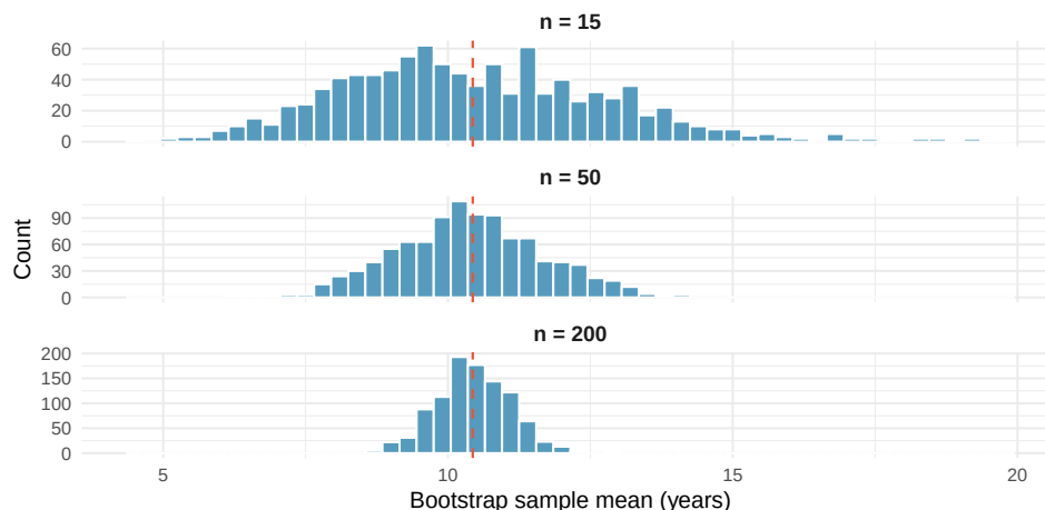
Figure 29: The effect of sample size on the bootstrap distribution. Larger samples produce narrower bootstrap distributions, leading to narrower confidence intervals. All three panels use the same population of penny ages.
