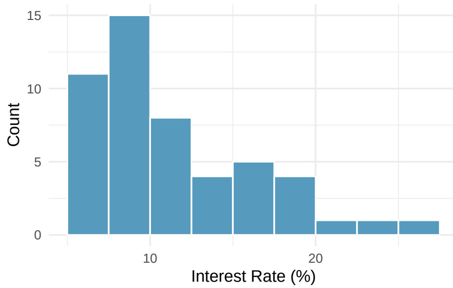
Figure 11: A histogram of interest rates with bin width 2.5 percentage points.
