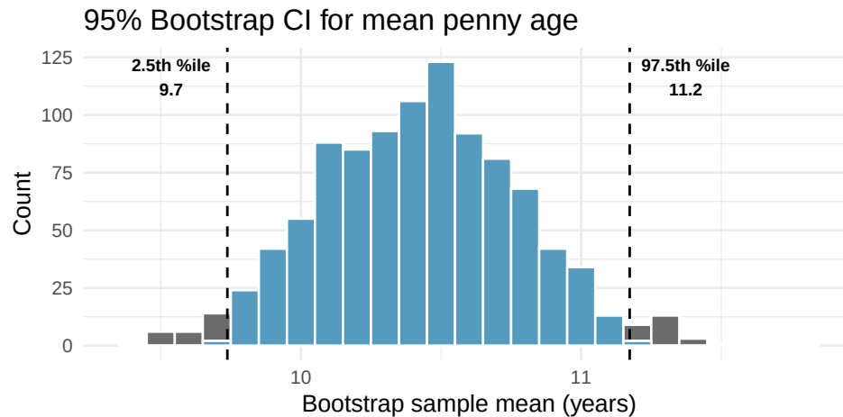
Figure 28: Bootstrap distribution of 1,000 sample means with the middle 95% shaded in blue. The 2.5th and 97.5th percentiles form the 95% confidence interval for the mean penny age.
