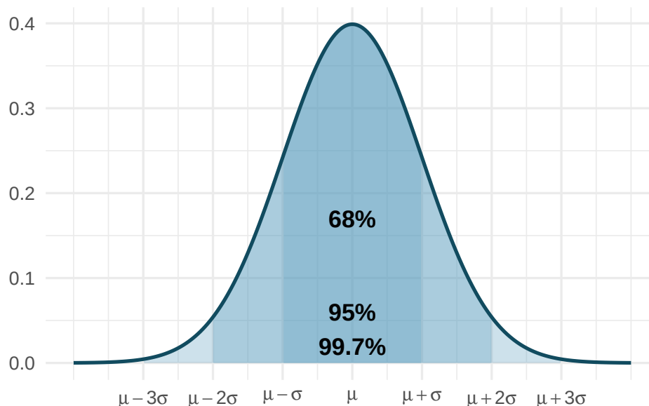
Figure 31: The 68-95-99.7 rule illustrated on a normal curve. The innermost shaded region (68%) extends from \mu - \sigma to \mu + \sigma . The middle region (95%) extends from \mu - 2\sigma to \mu + 2\sigma . The outermost region (99.7%) extends from \mu - 3\sigma to \mu + 3\sigma .
