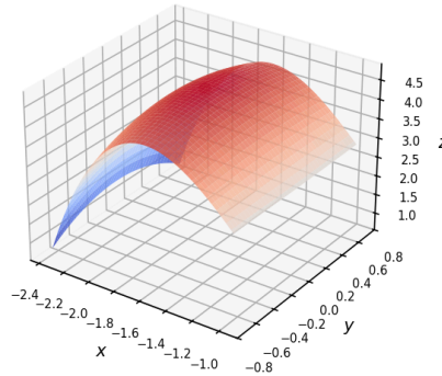
Local Maximum at (-\frac{5}{3}, 0) D > 0, f_{xx} < 0
