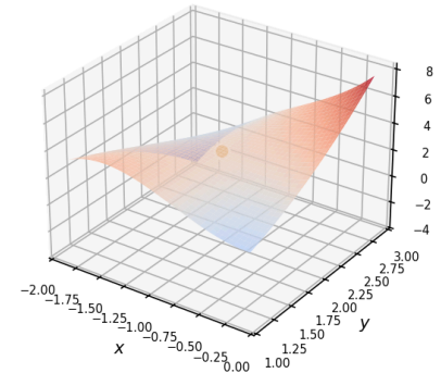
Saddle Point at (-1, 2) D < 0
