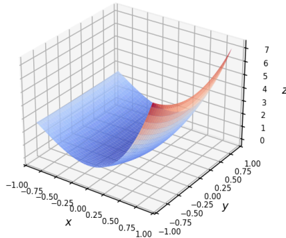
Local Minimum at (0, 0) D > 0, f_{xx} > 0
