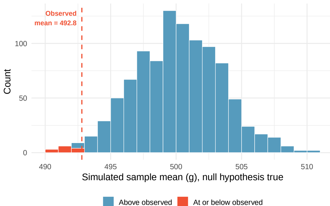
Figure 14.1: A histogram of 1,000 simulated sample means, each from a sample of 15 loaves drawn from data shifted to satisfy the null hypothesis (mean = 500 g). Simulated means at or below the observed 492.8 g are shaded in red.
