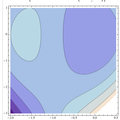
Contour plot of f | Desmos 3D [https://www.desmos.com/3d]
