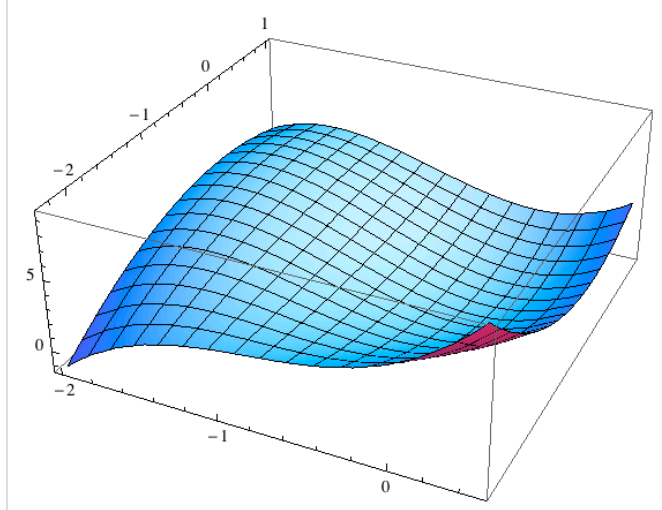
Surface plot of f | Desmos 3D [https://www.desmos.com/3d]
